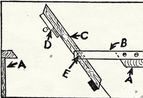
A Simple Type of Drawbridge
